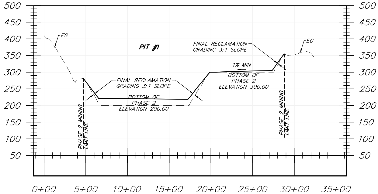
SECTION F SCALE: HORIZ 1"=700 VERT 1"=125'
