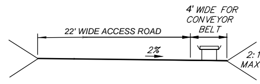
TYPICAL SECTION ACCESS ROAD AND CONVEYOR BELT NO SCALE
