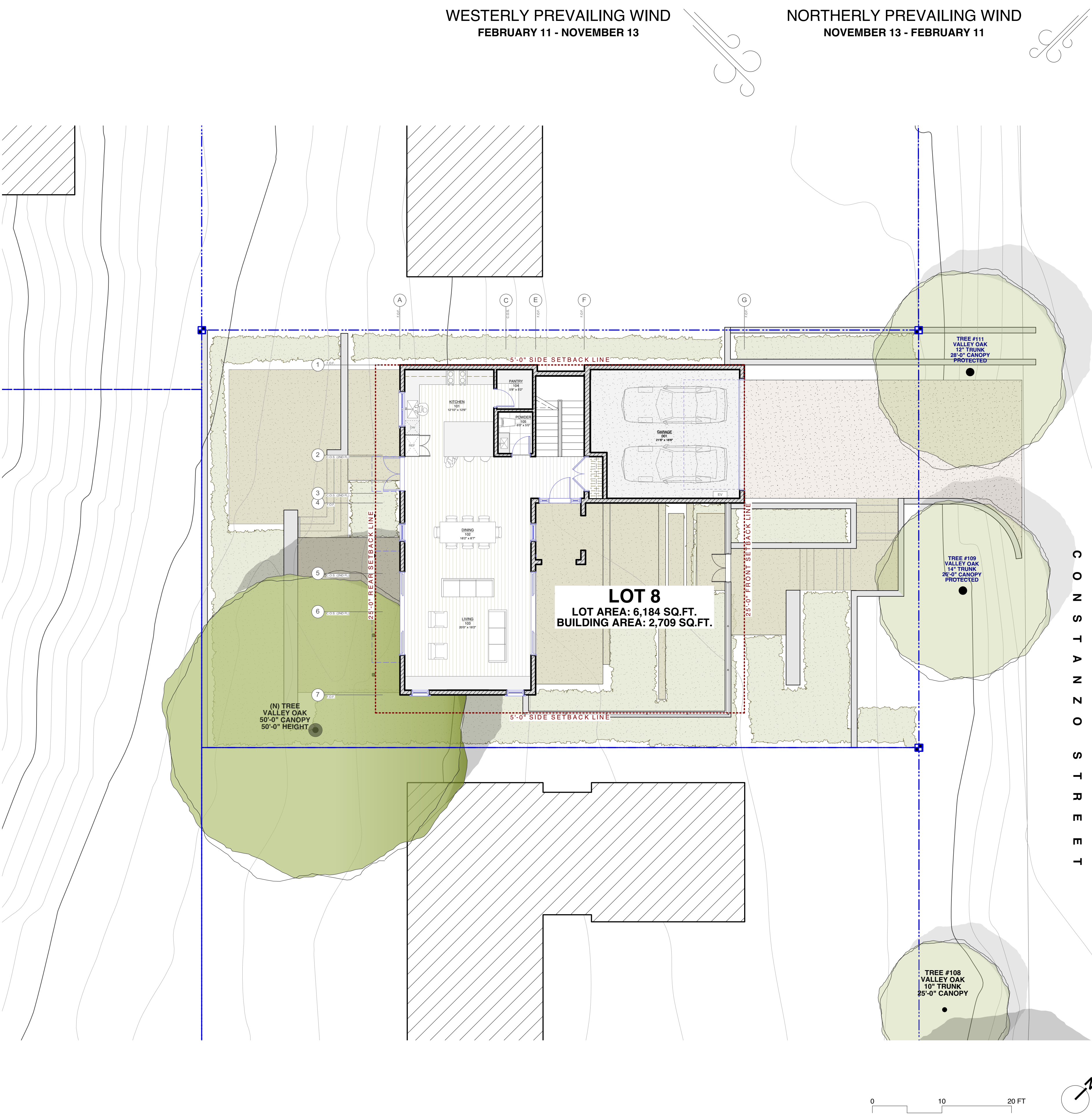
ENERGY CONSERVATION PLAN - LOT 8 Scale: 1/8" = 1'-0"
