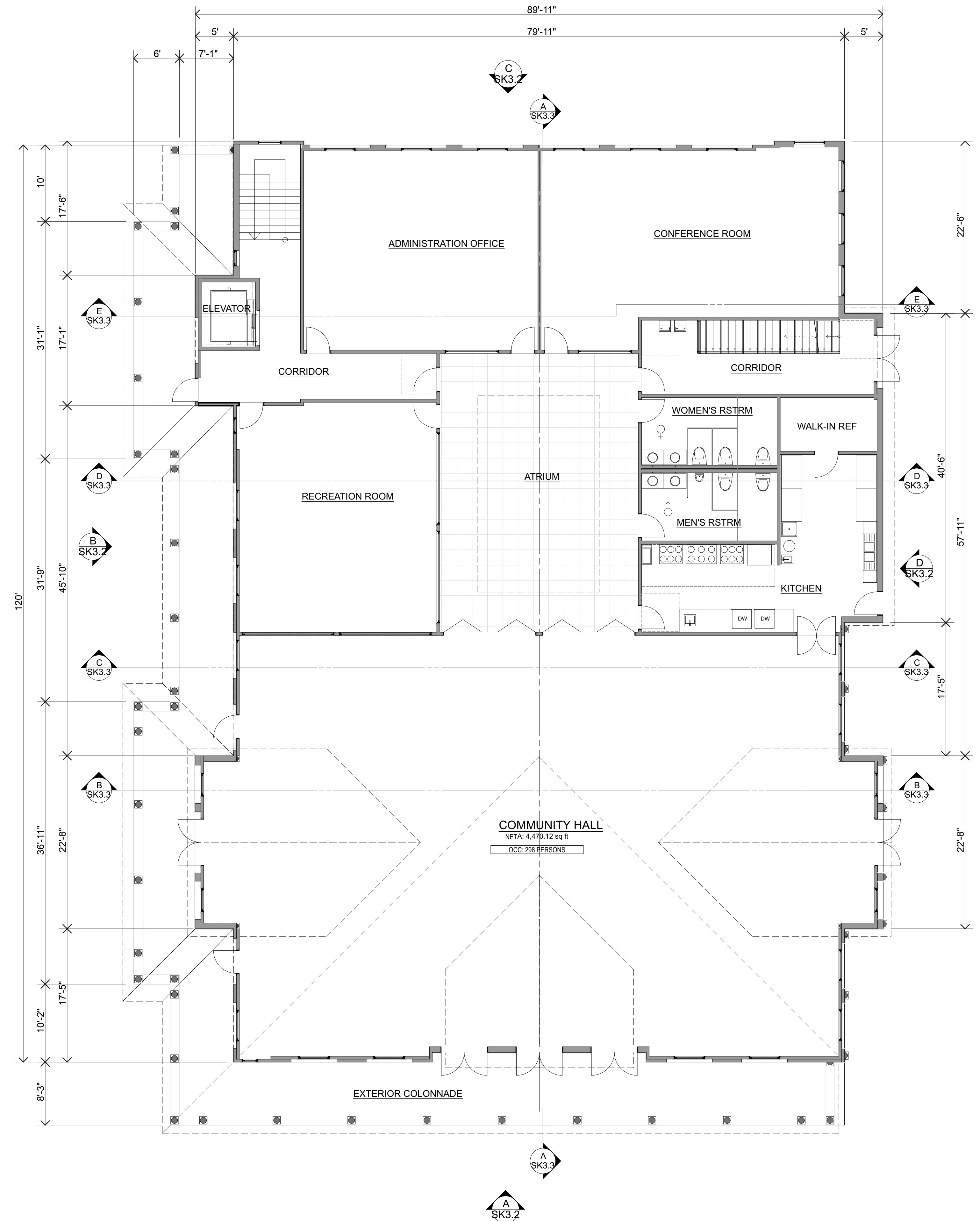
A SK3.1 COMMUNITY BUILDING FIRST FLOOR PLAN SCALE: 1/8" = 1'-0"
