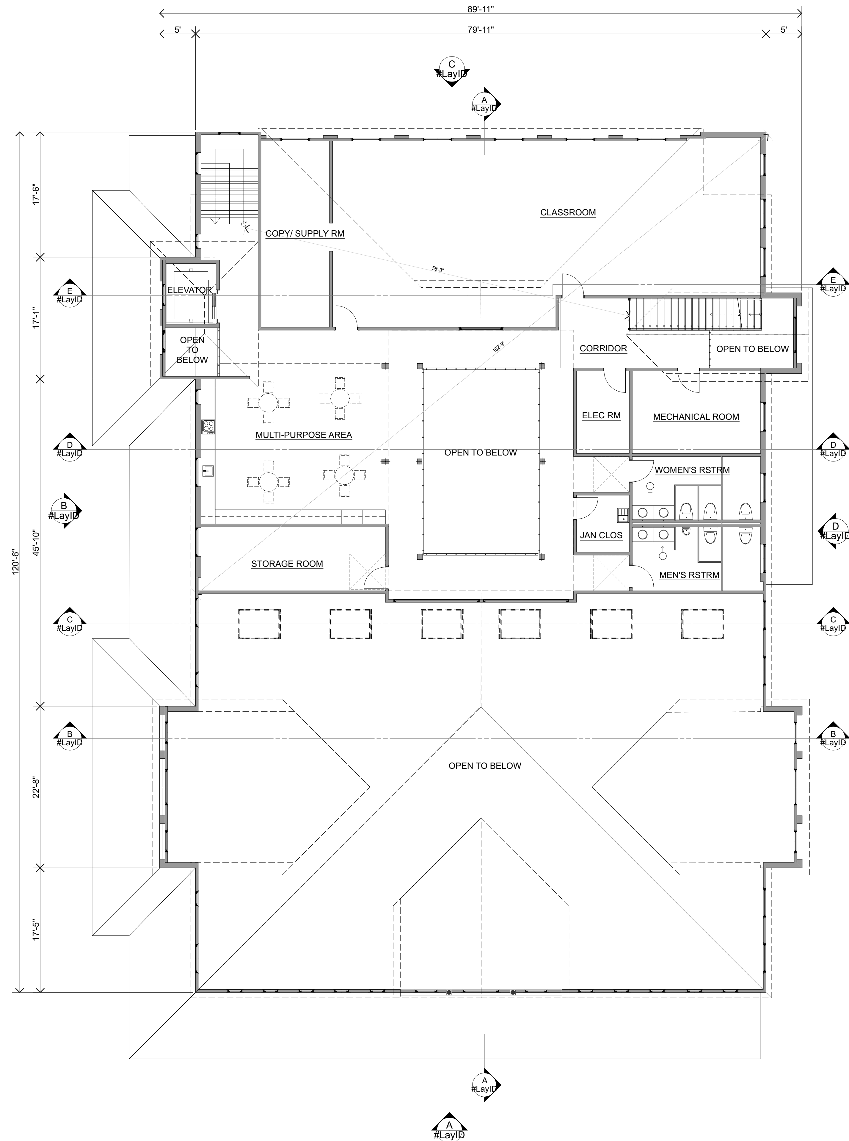
B SK3.1 COMMUNITY BUILDING SECOND FLOOR PLAN SCALE: 1/8" = 1'-0"
