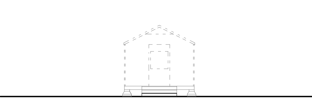
C.4 TENT FRONT ELEVATION SCALE: 1/8" = 1'-0"
