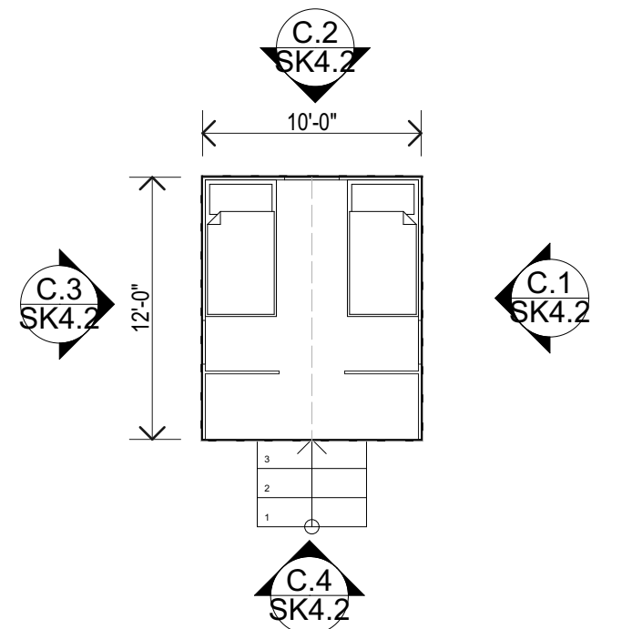
C TENT TYPICAL FLOOR PLAN SCALE: 1/8" = 1'-0"
