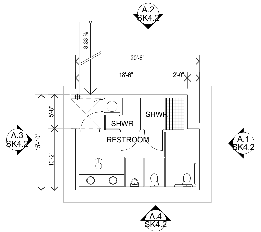
A BOY'S BATHHOUSE FLOOR PLAN SCALE: 1/8" = 1'-0"
