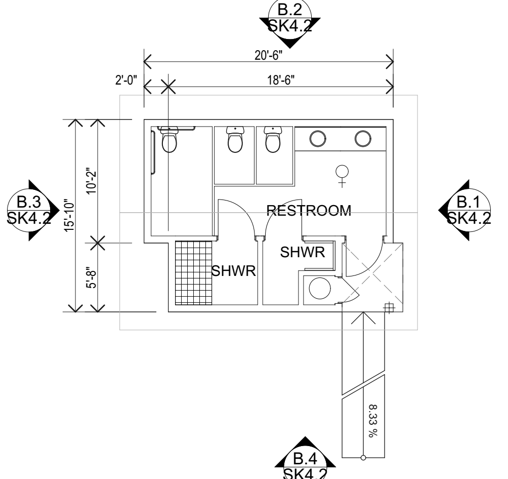
B GIRL'S BATHHOUSE FLOOR PLAN SCALE: 1/8" = 1'-0"
