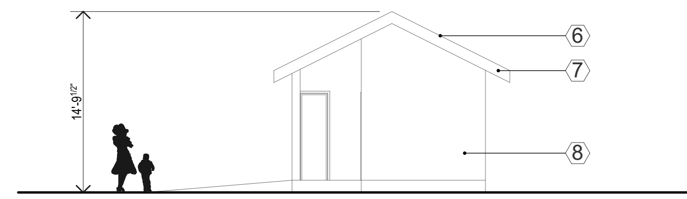
B.1 GIRL'S BATHHOUSE EAST ELEV SCALE: 1/8" = 1'-0"
