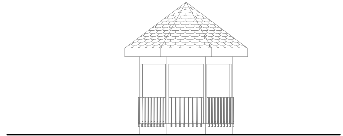
D.4 RAMADA SOUTH ELEVATION SCALE: 1/8" = 1'-0"
