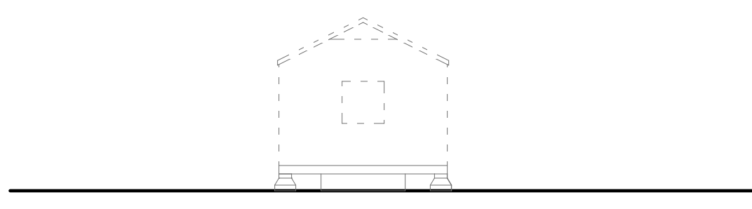
C.2 TENT REAR ELEVATION SCALE: 1/8" = 1'-0"
