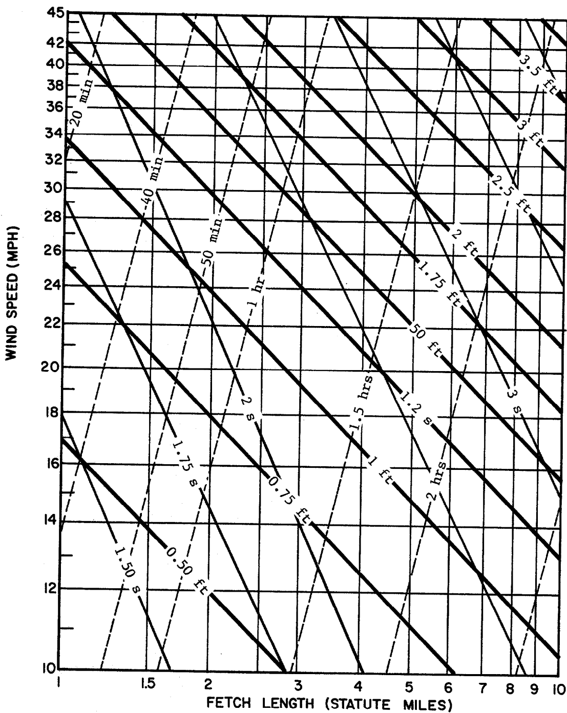
Chart 6. Nomograph of deepwater significant wave height prediction curves (modified from reference 29)
