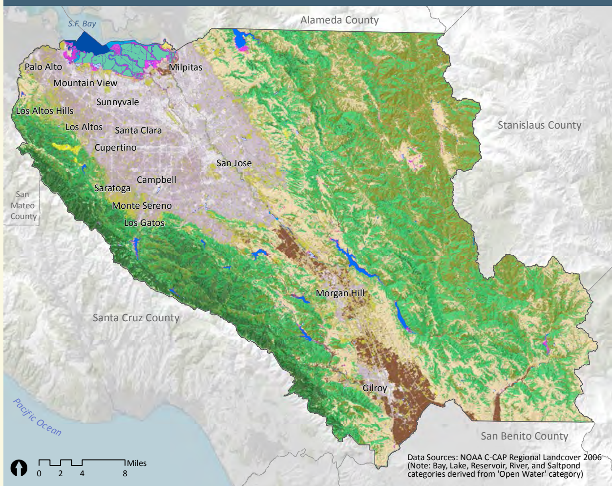
FIGURE 5: Land Cover in Santa Clara County
