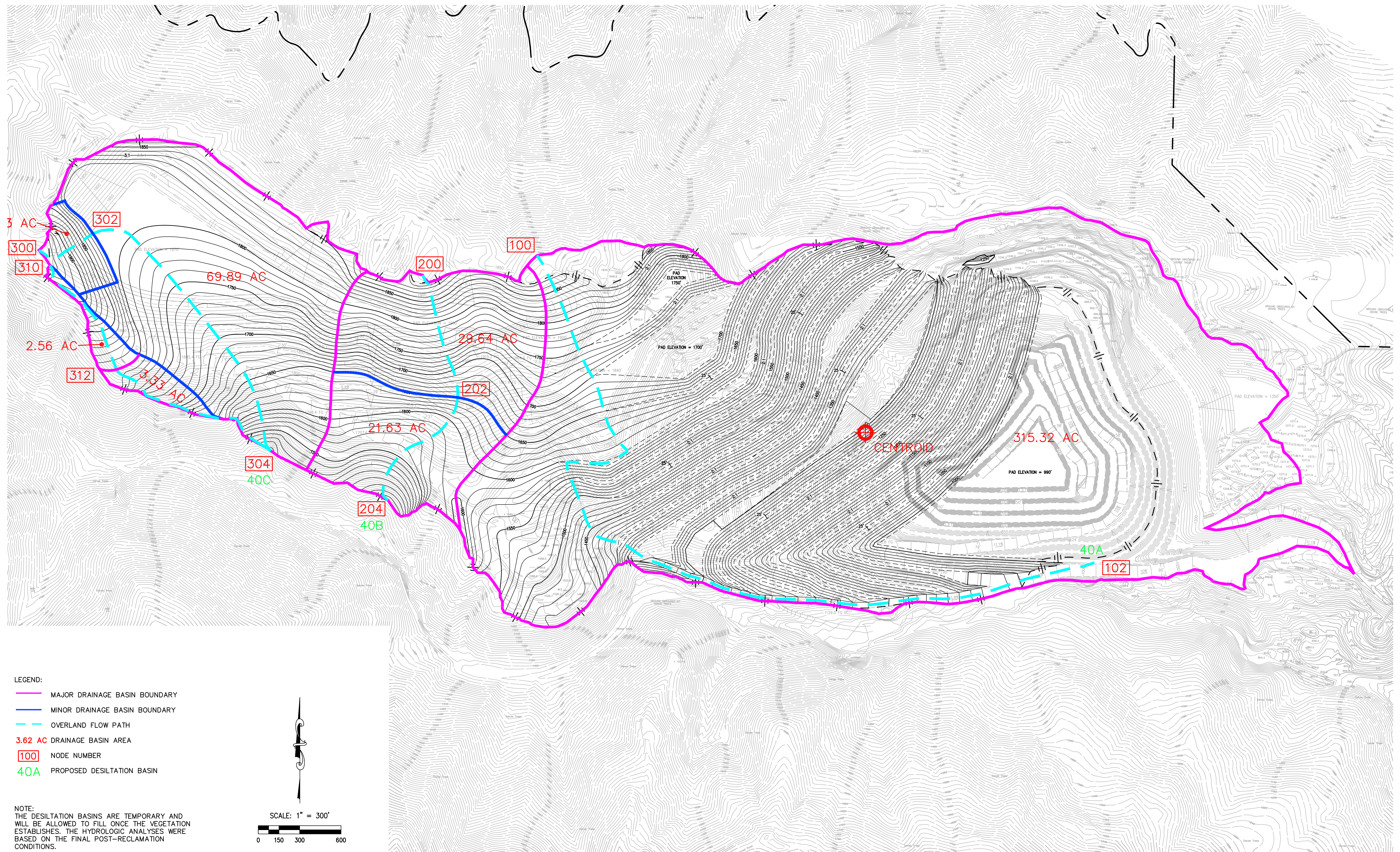
NORTH QUARRY & WEST MATERIALS STORAGE AREA PROPOSED CONDITION RATIONAL METHOD WORK MAP
