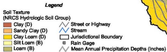
Figure 1 Soil Texture and Mean Annual Precipitation Depths for the Santa Clara Basin
