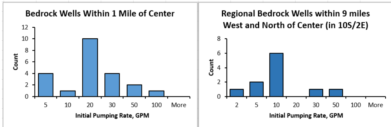
Figure E1 – Pumping Rates Reported on Well Logs for Initial Well Acceptance Tests
