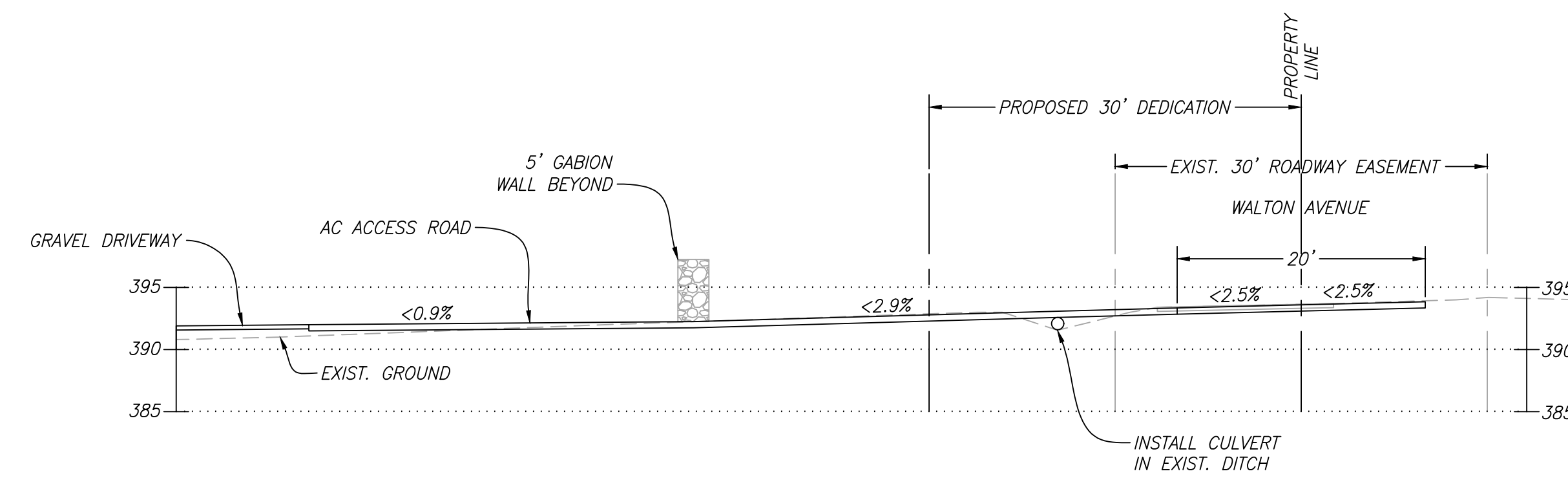
SECTION C-C
