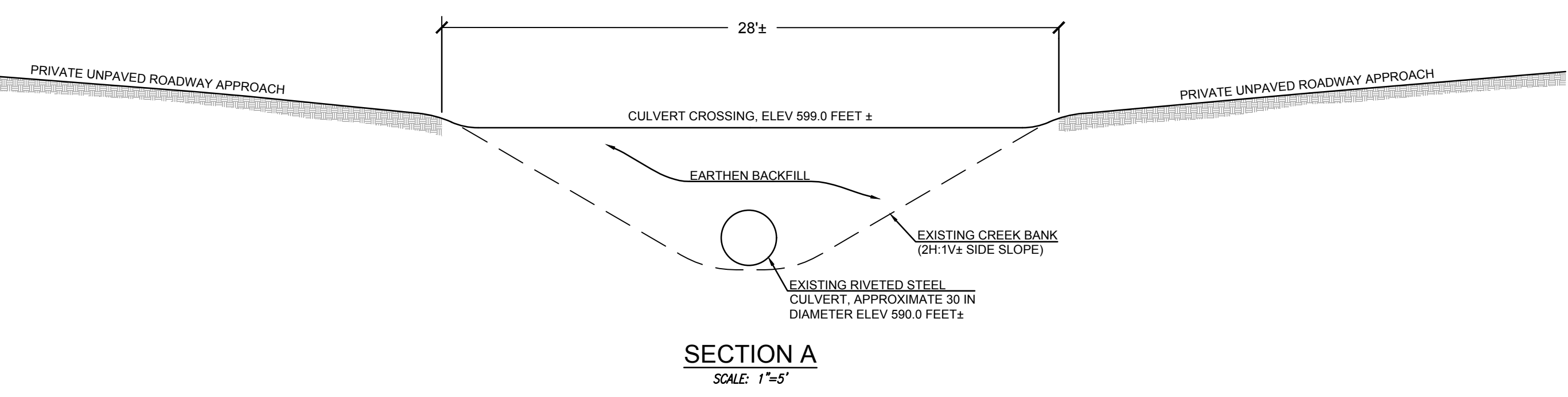
SECTION VIEW OF CULVERT CROSSING
