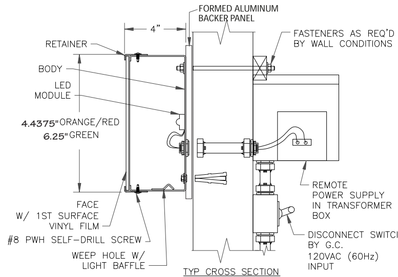
SECTION VIEW @TRI-STRIPLEILLUMINATED CHANNEL SET
