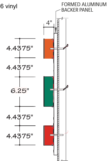
SIDE VIEW @ TRI-STRIPLE ILLUMINATED CHANNEL SET
