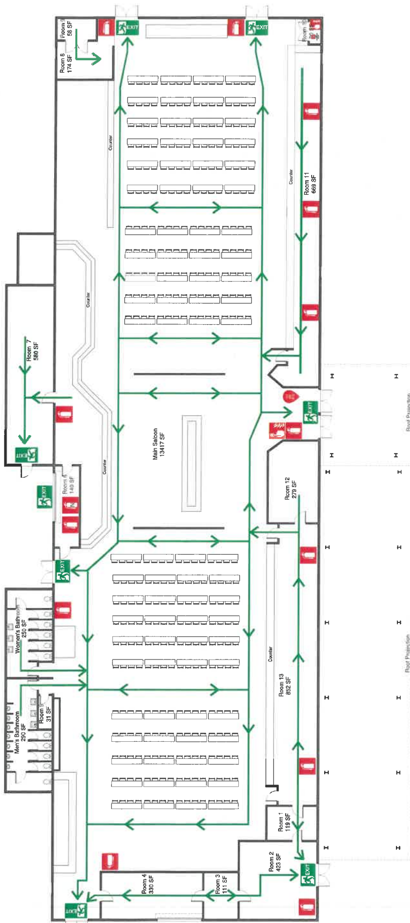
Fire Plan 1" = 6'-0"
