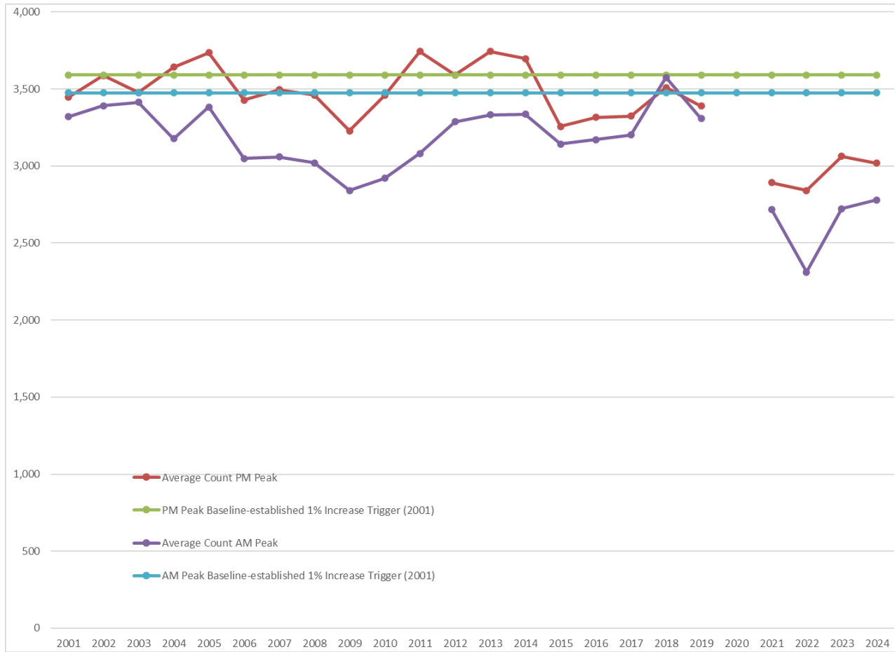
Figure 7 Peak-Hour (AM and PM) Traffic Volume Trends (Adjusted Traffic Data) 2001 - 2024
