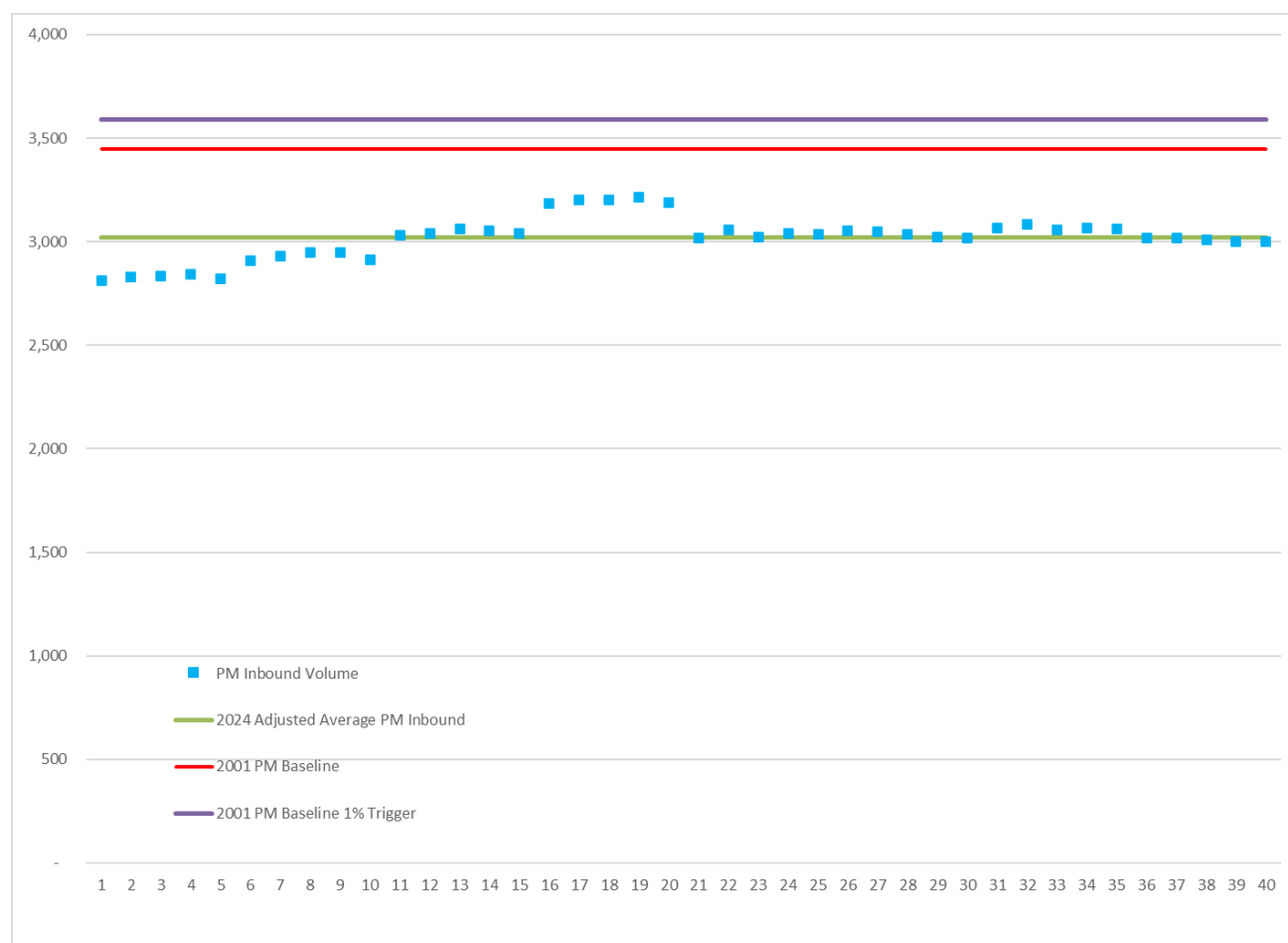
Figure 4 2024 PM Peak-Hour Adjusted Traffic Counts
